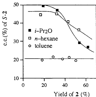
Fig. 3. Effect of solvent on the enantioselectivity of acetylation of (±)-1 by Pseudomonas sp. lipase.
