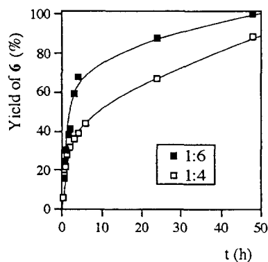
Fig. 8. Progress curves for acylation of S - 1 with 4 at different molar ratios 4 : S - 1 (e.e. 42.5%) in n -hexane.
