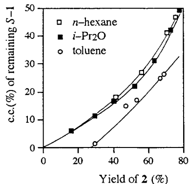
Fig. 6. Effect of solvent on the enantioselectivity of acetylation of (±)-1 by Penicillium camembertii lipase.
