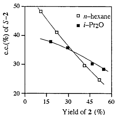
Fig. 5. Effect of solvent on the enantioselectivity of acetylation of (±)-1 by Lipozyme IM lipase.
