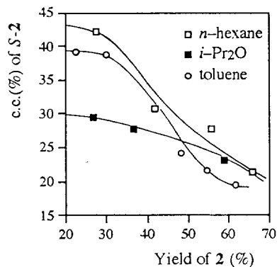
Fig. 4. Effect of solvent on the enantioselectivity of acetylation of (±)-1 by lipase from hog pancreas.
