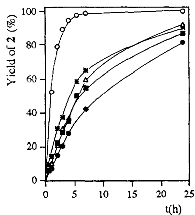
Fig. 2. Progress curves for acetylation of ( \pm )-1 with lipases in diisopropylether
