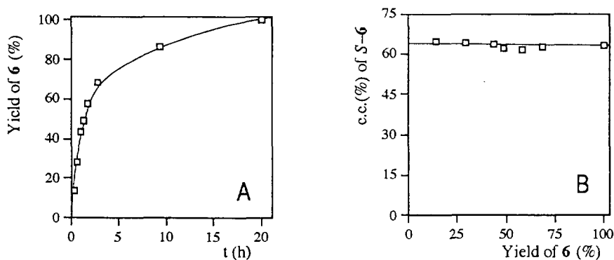
Fig. 7. Conversion (A) and enantioselectivity (B) in transesterification of (±)- 1 by vinylcinnamate 4 in n -hexane.
