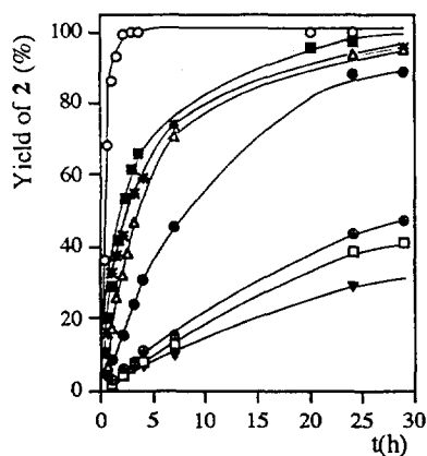
Fig. 1. Progress curves for acetylation of ( \pm )-1 with lipases in n -hexane.
